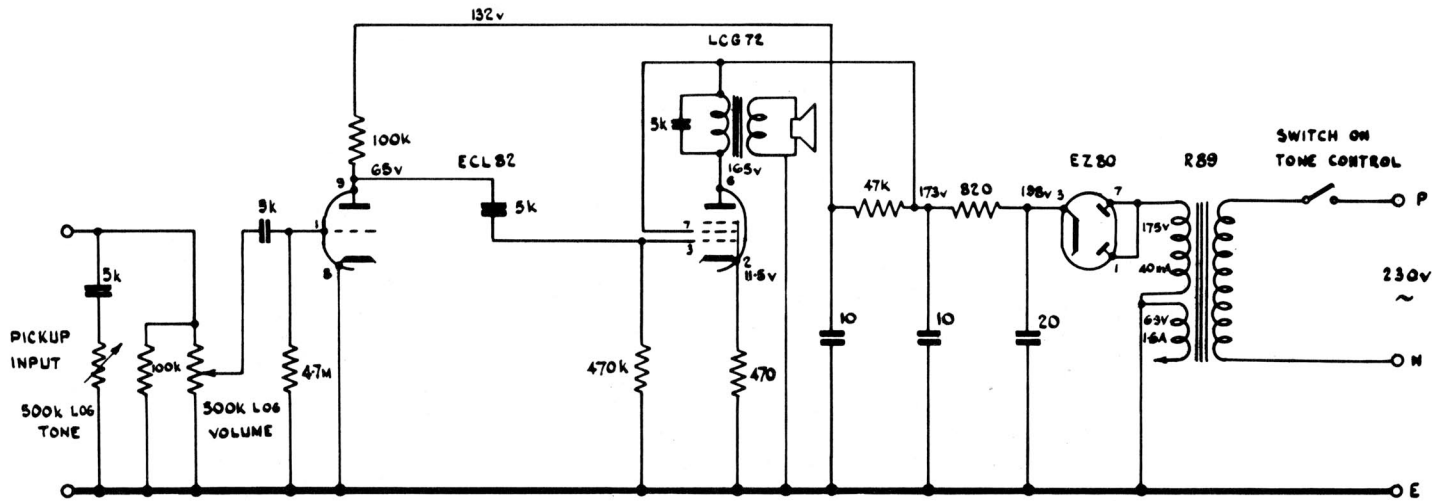
A.C. PLAYER CIRCUIT DIAGRAM
